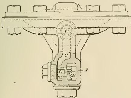
Fig. 1a.—VALVE FOR TRIPLE VALVE TESTING DEVICE.
